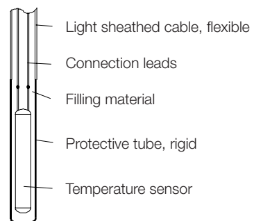
Construction of a sheath resistance thermometer
