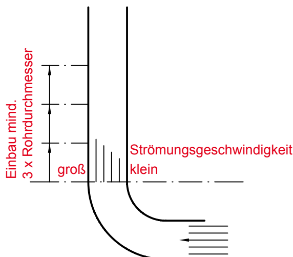
Mounting position fig. 3
