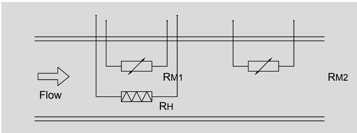
Measuring principle Fig. 1
